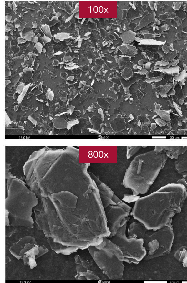
Scanning Electron Microscopy images at 100x and 800x magnification showing clean, pure crystalline flake structure
